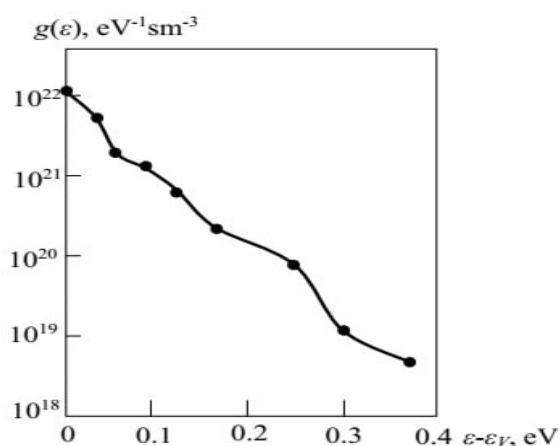
Fig. 3. The distribution of the density of electronic states at the tail of the valence band for amorphous Se 0.5 S 0.5 was obtained from formula (12).
