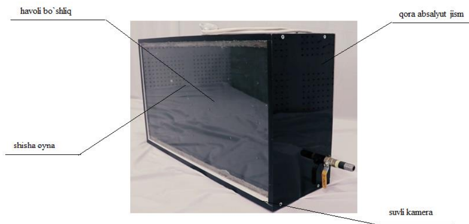
1-rasm. Suv isitish qurilmasining tashqi ko‘rinishi
