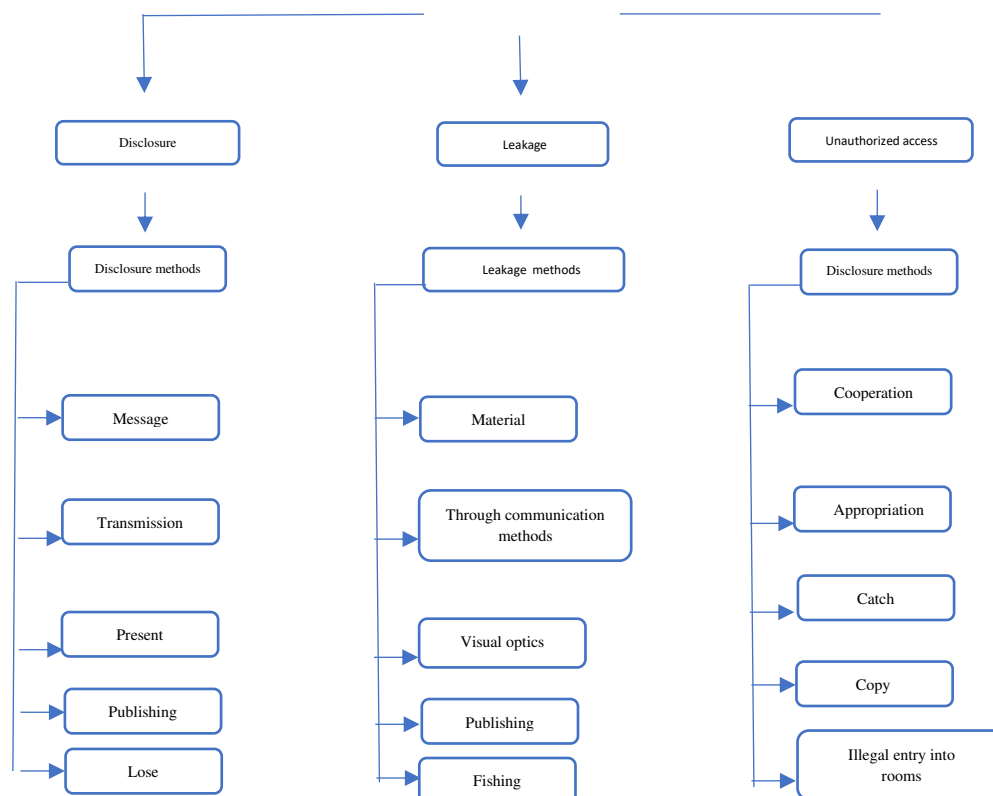
3- picture. Methods of loss of confidential information.
